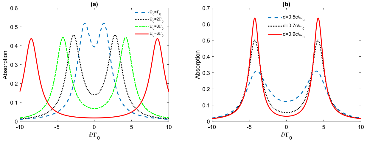
Fig. 2. The absorption spectrum [\chi''] of the ladder-shaped light-matter quantum coupling (in units of \frac{N\mu_{10}^2}{\epsilon_0\hbar} ) versus the detuning of probe field \delta . (a) is when the plasmonic nanostructure is absent ( d = \infty ), while (b) is in the presence of the plasmonic nanostructure. In (a), the decay rate is \Gamma_0 , but in (b) \bar{\omega} = 0.632\omega_p . In (a) the spectrum is plotted for different values of the control field, i.e., \Omega_c = \Gamma_0 (dashed blue), \Omega_c = 2\Gamma_0 (dotted black), \Omega_c = 3\Gamma_0 (dashed-dotted green) and \Omega_c = 6\Gamma_0 (red solid). In (b) the spectrum is plotted for \Omega_c = 3\Gamma_0 and for different distances d between the emitter and the surface of the plasmonic nanostructure, i.e., d = 0.5c/\omega_p (dashed blue), d = 0.7c/\omega_p (dotted black) and d = 0.9c/\omega_p (red solid).
