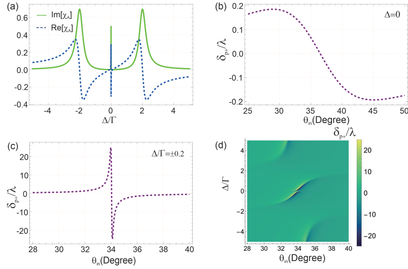
Fig. 5. (a) Optical susceptibility versus the normalized probe detuning \Delta/\Gamma , where the absorptive response is indicated by a solid curve and the dispersive response by a dashed curve. (b) Transverse photonic spin Hall shift \delta_{p+} as a function of the incidence angle \theta_{in} for resonant probe detuning i.e. \Delta = 0 . (c) The corresponding \delta_{p+}-\theta_{in} dependence by considering detuning \Delta = \pm 0.2\Gamma . (d) Density plot of PSHE \delta_{p+}-\theta_{in} as a function of the incidence angle \theta_{in} and detuning \Delta/\Gamma . The set of parameters used is: \Gamma = 1 MHz, \phi = 0 , \theta = 0 , \delta = 0.1\Gamma , |\Omega_{A0}| = |\Omega_{B0}| = 0.1\Gamma , and \Omega = \Gamma . Constants and optical quantities are taken as \epsilon_0 = 8.85 \times 10^{-12} F/m, \hbar = 1.05 \times 10^{-34} J · s, \mathbf{d}_{A0} = \mathbf{d}_{B0} = 1.269 \times 10^{-29} C m, atomic density N/V = 10^{12} m ^{-3} , \lambda = 852 nm, and k_0 = 2\pi/\lambda . A Gaussian beam with waist \omega_0 = 50\lambda and parameter q = 0.1 \times 10^{-6} m is assumed, and the dielectric constants are \epsilon_1 = \epsilon_3 = 2.22 and \epsilon_2 = 1 + \chi_A(\omega_p) .
