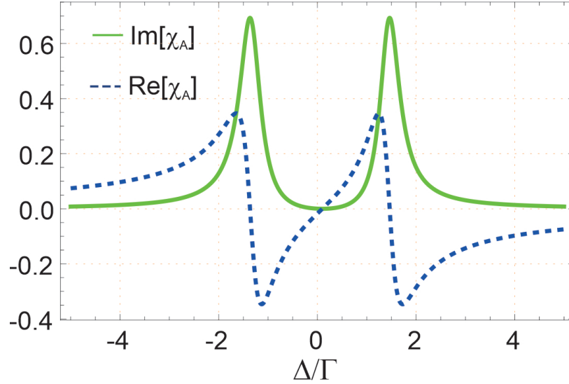
Fig. 2. Real (dashed curve) and imaginary (solid curve) components of the optical susceptibility as functions of the normalized probe detuning \Delta/\Gamma . Unless stated otherwise, the numerical values used are: \Gamma = 1 MHz, \delta = 0.1\Gamma , \phi = \pi , \theta = 0 , \Omega = \Gamma , \epsilon_0 = 8.85 \times 10^{-12} F/m, an atomic number density N/V = 10^{12} m ^{-3} , \hbar = 1.05 \times 10^{-34} J \cdot s, d_{A0} = 1.269 \times 10^{-29} C m.
