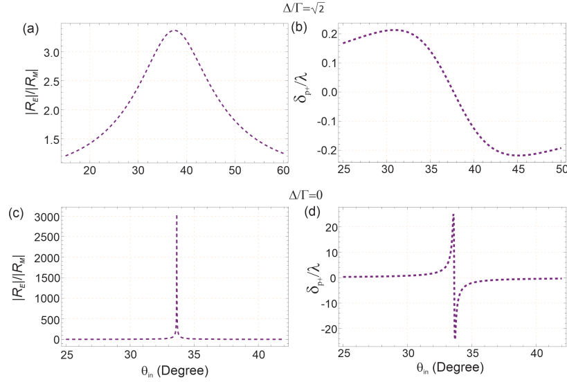
Fig. 3. Dependence of the reflection-coefficient magnitude ratio |R_E/R_M| on the incidence angle \theta_{in} for (a) \Delta/\Gamma = \sqrt{2} , and (c) \Delta/\Gamma = 0 . The associated PSHE displacement \delta_{p+}/\lambda as a function of \theta_{in} is shown in (b) \Delta/\Gamma = \sqrt{2} , and (d) \Delta/\Gamma = 0 . Unless otherwise stated, the parameters are \Gamma = 1 MHz, \delta = 0.1\Gamma , \phi = \pi , \theta = 0 , probe-field amplitudes |\Omega_{A0}| = |\Omega_{B0}| = 0.1\Gamma , \Omega = \Gamma , \epsilon_0 = 8.85 \times 10^{-12} F/m, \hbar = 1.05 \times 10^{-34} J · s, atomic density N/V = 10^{12} m ^{-3} , dipole moment \mathbf{d}_{A0} = 1.269 \times 10^{-29} C m, wavelength \lambda = 852 nm, wave number k_0 = 2\pi/\lambda , beam waist \omega_0 = 50\lambda , q = 0.1 \times 10^{-6} m, and permittivities \epsilon_1 = \epsilon_3 = 2.22 , with \epsilon_2 = 1 + \chi_A(\omega_p) .
