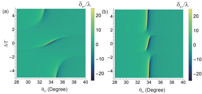
Fig. 4. (a) Transverse photonic spin Hall displacement \delta_{p+} plotted against the incidence angle \theta_{in} for a density N/V = 10^{12} m ^{-3} . (b) The corresponding \delta_{p+}-\theta_{in} characteristic when the density is reduced by one decade to N/V = 10^{11} m ^{-3} . The calculations are performed using \Gamma = 1 MHz, \delta = 0.1\Gamma , \phi = \pi , \theta = 0 , probe-field amplitudes |\Omega_{A0}| = |\Omega_{B0}| = 0.1\Gamma , and \Omega = \Gamma . Other constants are \epsilon_0 = 8.85 \times 10^{-12} F/m, \hbar = 1.05 \times 10^{-34} J · s, \mathbf{d}_{A0} = \mathbf{d}_{B0} = 1.269 \times 10^{-29} C m, \lambda = 852 nm, and k_0 = 2\pi/\lambda . The Gaussian beam parameters are \omega_0 = 50\lambda and q = 0.1 \times 10^{-6} m. The dielectric environment is defined by \epsilon_1 = \epsilon_3 = 2.22 and \epsilon_2 = 1 + \chi_A(\omega_p) .
