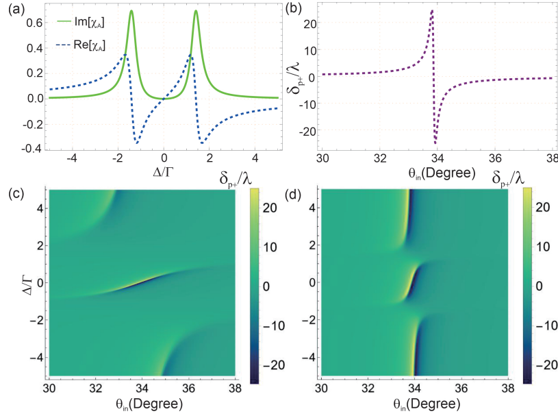
Fig. 6. (a) Dependence of the medium susceptibility on the normalized probe detuning \Delta/\Gamma , where the solid (dashed) trace represents the absorptive (dispersive) component. (b) Transverse photonic spin Hall shift \delta_{p+} as a function of the incidence angle \theta_{in} for resonant probe detuning \Delta = 0 and N/V = 10^{12} \text{ m}^{-3} . (c) Density plot of photonic spin Hall shift \delta_{p+} as a function of the incidence angle \theta and probe detuning \Delta/\Gamma for N/V = 10^{12} \text{ m}^{-3} . (d) The same quantity \delta_{p+} versus \theta_{in} when the number density is decreased by one decade to N/V = 10^{11} \text{ m}^{-3} . The calculations assume \Gamma = 1 \text{ MHz} , \delta = 0 , \phi = \pi , \theta = 0 , probe amplitudes |\Omega_{A0}| = |\Omega_{B0}| = 0.1\Gamma , and \Omega = \Gamma . Further constants are \epsilon_0 = 8.85 \times 10^{-12} \text{ F/m} , \hbar = 1.05 \times 10^{-34} \text{ J} \cdot \text{s} , \mathbf{d}_{A0} = \mathbf{d}_{B0} = 1.269 \times 10^{-29} \text{ C m} , \lambda = 852 \text{ nm} , and k_0 = 2\pi/\lambda . A Gaussian beam with waist \omega_0 = 50\lambda and parameter q = 0.1 \times 10^{-6} \text{ m} is used. The dielectric constants are chosen as \epsilon_1 = \epsilon_3 = 2.22 and \epsilon_2 = 1 + \chi_A(\omega_p) .
