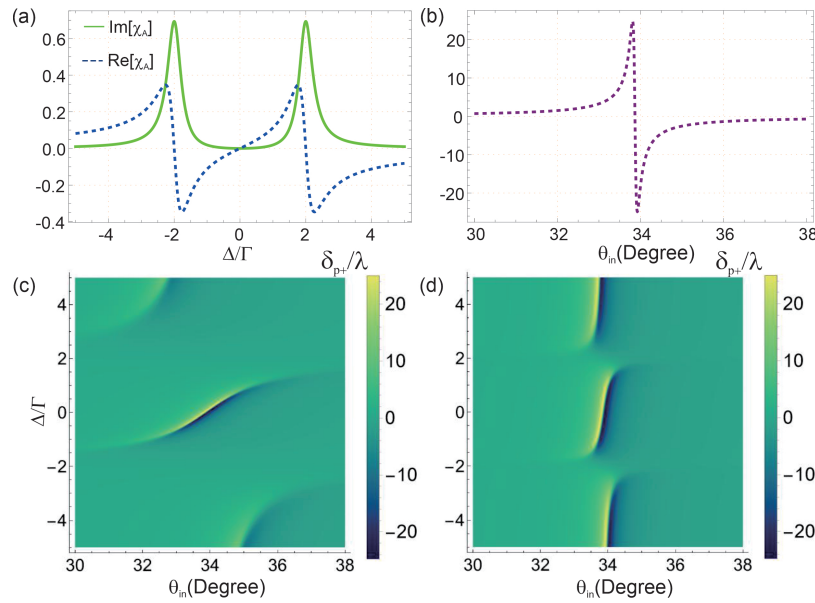
Fig. 7. (a) Absorption (solid curve) and dispersion (dashed curve) of the susceptibility as functions of the scaled probe detuning \Delta/\Gamma . (b) Transverse photonic spin Hall shift \delta_{p+} versus incidence angle \theta_{in} for \Delta = 0 and a number density N/V = 10^{12} \text{ m}^{-3} . (c) Density plot of photonic spin Hall shift \delta_{p+} versus incidence angle \theta_{in} and probe detuning \Delta/\Gamma for a number density N/V = 10^{12} \text{ m}^{-3} . (d) The same angular dependence of \delta_{p+} when the density is reduced by one decade to N/V = 10^{11} \text{ m}^{-3} . The parameter set used is: \Gamma = 1 \text{ MHz} , \delta = 0 , \phi = 0 , \theta = 0 , |\Omega_{A0}| = |\Omega_{B0}| = 0.1\Gamma , and \Omega = \Gamma , together with \epsilon_0 = 8.85 \times 10^{-12} \text{ F/m} , \hbar = 1.05 \times 10^{-34} \text{ J} \cdot \text{s} , \mathbf{d}_{A0} = \mathbf{d}_{B0} = 1.269 \times 10^{-29} \text{ C m} , \lambda = 852 \text{ nm} , and k_0 = 2\pi/\lambda . A Gaussian beam is assumed with \omega_0 = 50\lambda and q = 0.1 \times 10^{-6} \text{ m} . The dielectric constants are taken as \epsilon_1 = \epsilon_3 = 2.22 and \epsilon_2 = 1 + \chi_A(\omega_p) .
