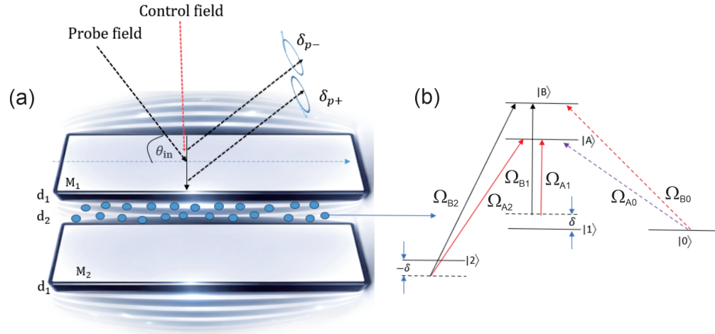
Fig. 1. (a) Schematic of a three-layer cavity comprising two mirrors, M_1 and M_2 , with a double-tripod (DT) atomic medium placed between them. When a TM-polarized probe beam of Rabi-frequency \Omega_{A0} is incident on M_1 , the reflected field experiences a spin-dependent spatial splitting. (b) Double-tripod level scheme, in which three ground states |0\rangle , |1\rangle , and |2\rangle are coupled to two excited states |A\rangle and |B\rangle . The system is driven by two probe fields \Omega_{A0} and \Omega_{B0} , along with four strong control fields \Omega_{A1} , \Omega_{B1} , \Omega_{A2} , and \Omega_{B2} .
